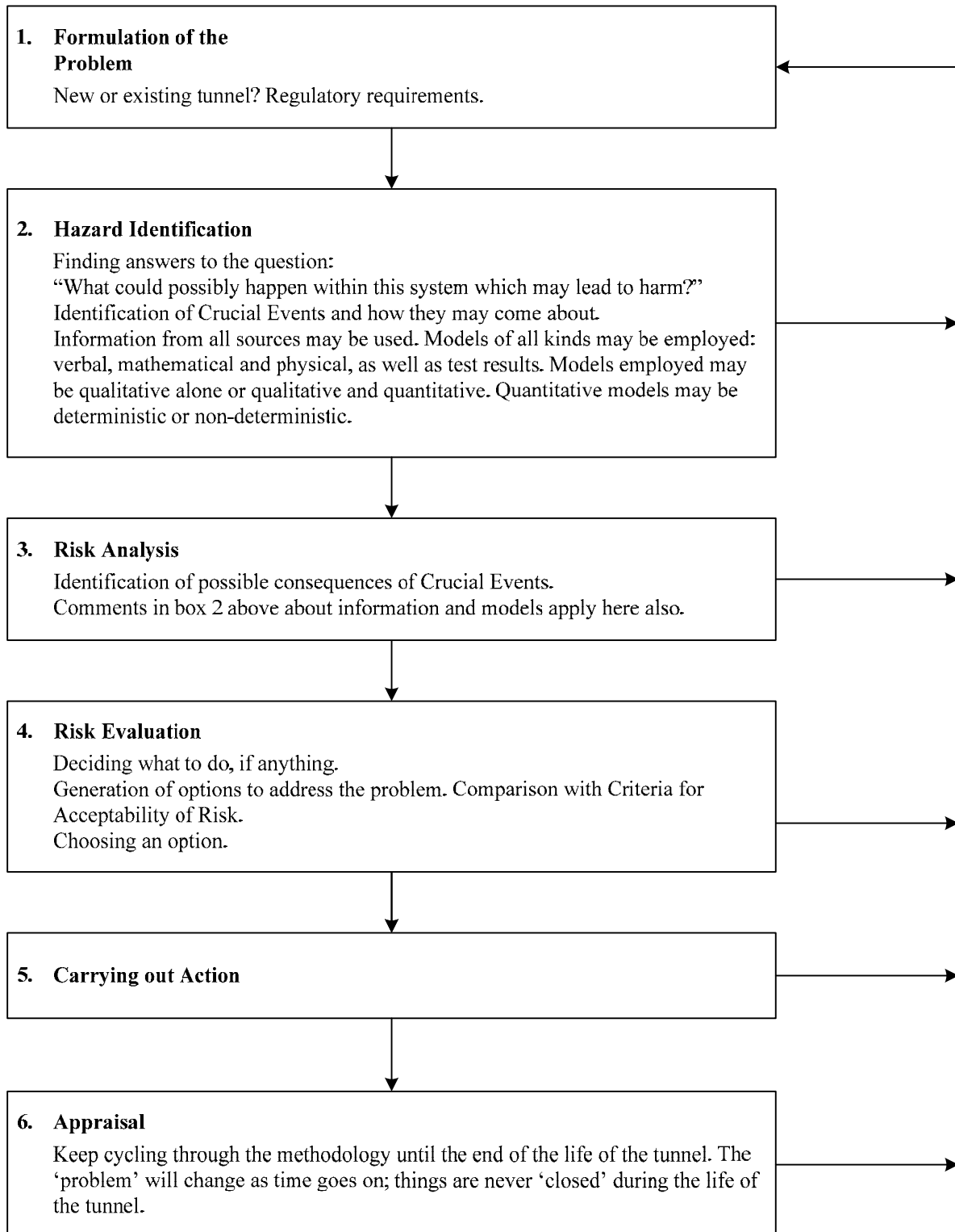
Figure 7: A generic methodology for design including risk assessment (In applying such a methodology the features identified with the bullet points in Section 3.3 should be put into effect); copyright A. N. Beard
