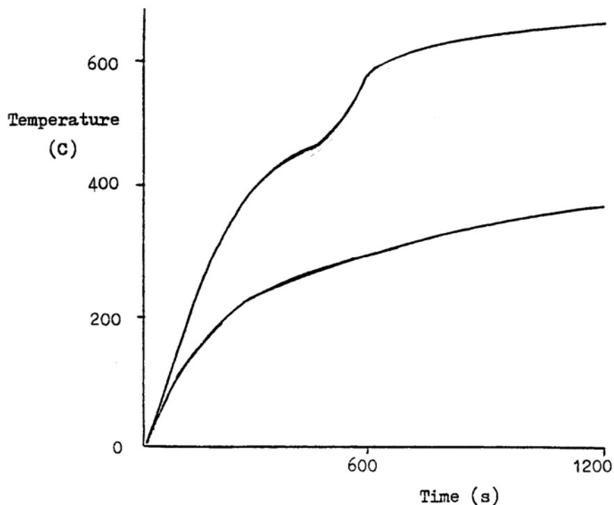
Figure 8: Ostensibly ‘identical’ tests; results from two experiments intended to be the same (copyright A. N. Beard)
