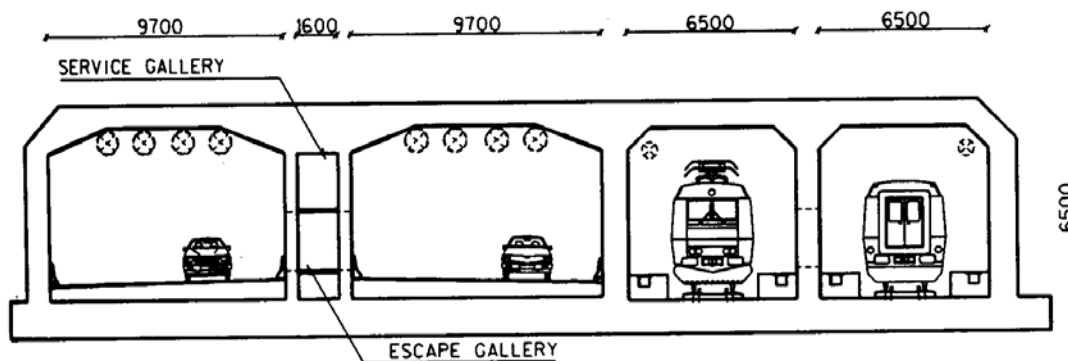
Figure 14: The Oresund Link: cross-section of the Drogden Tunnel (Distances shown in millimetres)
