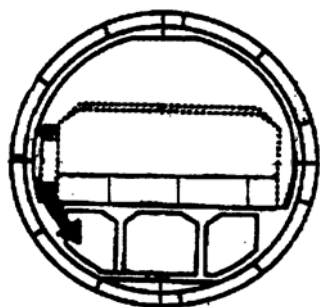
Figure 15: Trans Tokyo Bay Tunnel: cross-section of one tube of a twin-tube tunnel; illustrating the general principle of a slide (arrow) from the road-way level to an evacuation space below.
