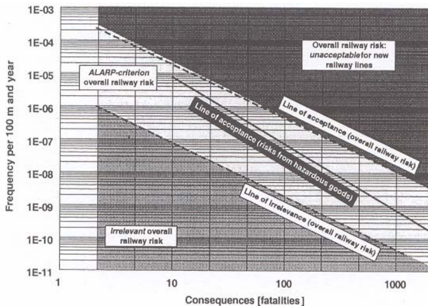
Figure 11: Societal Risk Criteria for the Gotthard Base Tunnel (F-N Curves) (Note: 1E-03 means 1(10^{-3}) i.e. 1/1000 and likewise)
